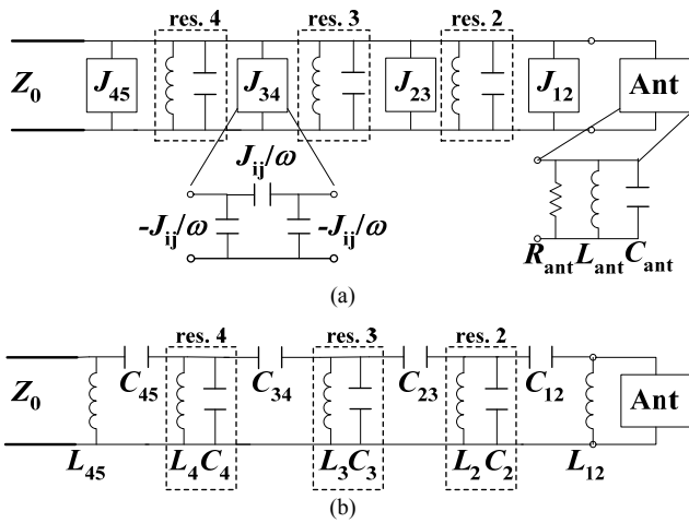
Fig. 10. (a) Illustration and (b) corresponding implementation of the impedance matching network using filter design techniques [21] for the loaded HF slot-loop antenna. Four-pole prototype matching circuit (including the antenna) is used in this case.
